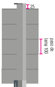
Paneles ciegos Ranch PB09 (100)
