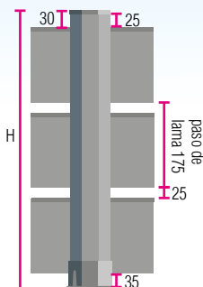
Paneles venecianos CL07 (136)
